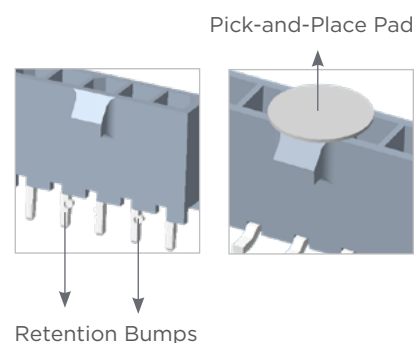
Retention Bumps
