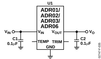
Figure 34. Basic Configuration
