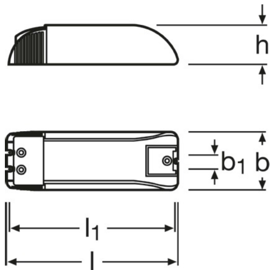
Product line drawing OTe 35/220...240/700 PC
