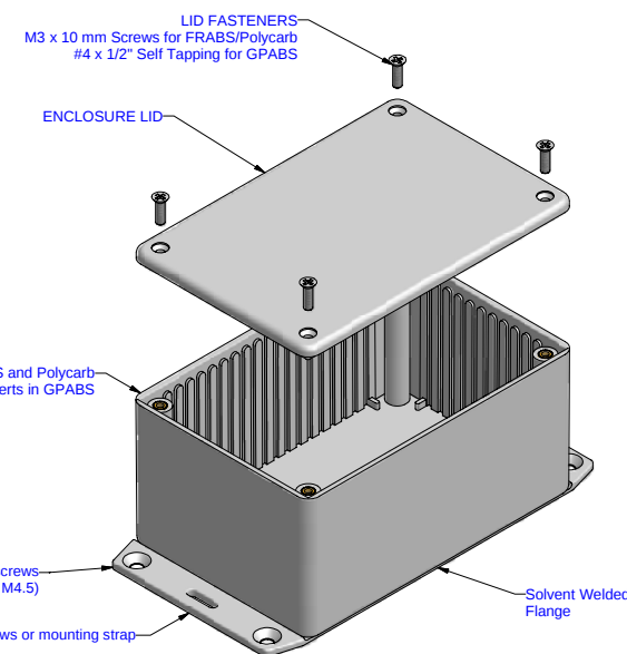
EXPLODED VIEW OF ASSEMBLY
