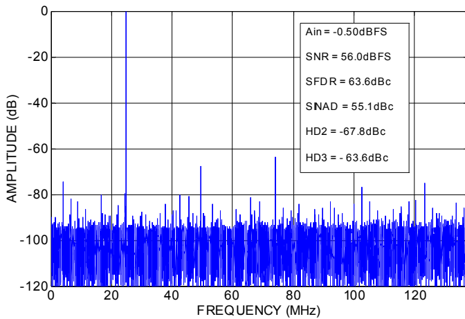
FIGURE 15. OUTPUT SPECTRUM; f_{\text{IN}} = 300\text{MHz}
