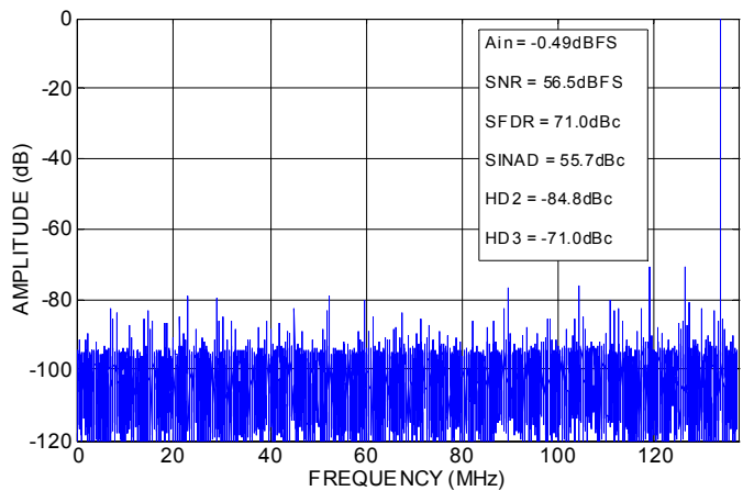
FIGURE 14. OUTPUT SPECTRUM; f_{\text{IN}} = 134\text{MHz}
