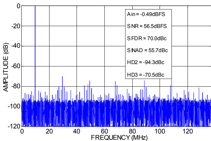
FIGURE 13. OUTPUT SPECTRUM; f_{\text{IN}} = 10\text{MHz}
