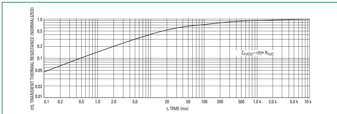
Figure 8. Thermal Response
