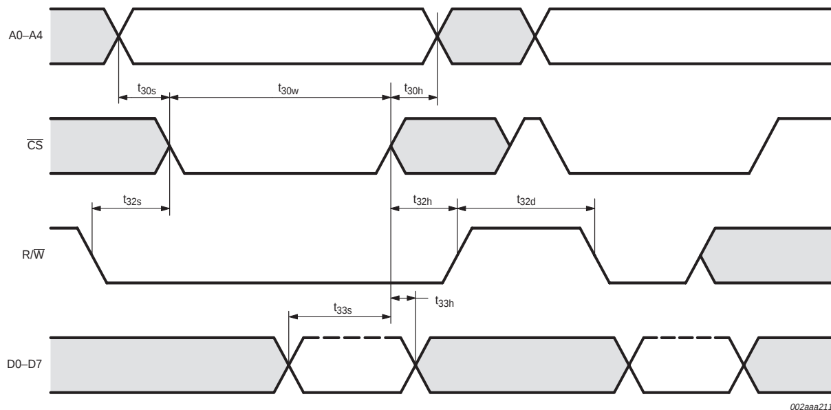
Fig 10. General write timing in 68 mode.
