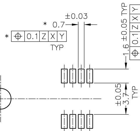
DETAIL A (4:1)
