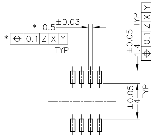
REFERENTIAL METAL MASK PAD OPENING (4:1)
