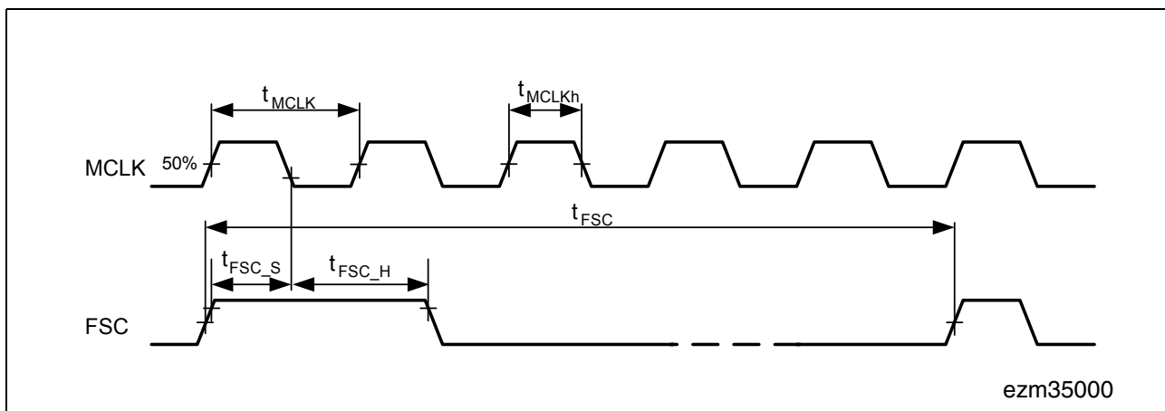
Figure 84 MCLK/FSC-Timing
