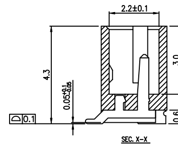
SEC. X-X
