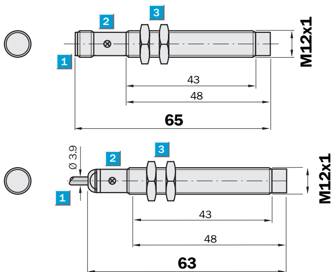
Dimensional drawing
