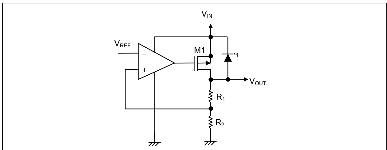
Figure 17 Voltage regulator circuit
