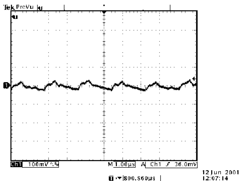
Ripple and noise at full load and 12.0Vdc input, and T_a=25^{\circ}\text{C} with 560 μF external cap
