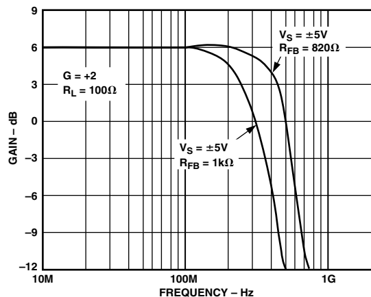
TPC 7. Frequency Response, G = +2
