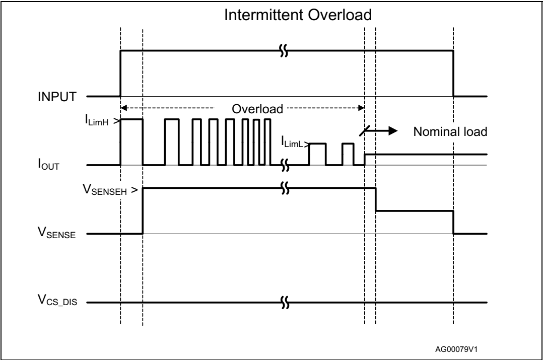
Figure 13. Intermittent overload
