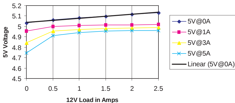
Figure 2. BLP55-3000 5V Output Voltage vs. 12V load
