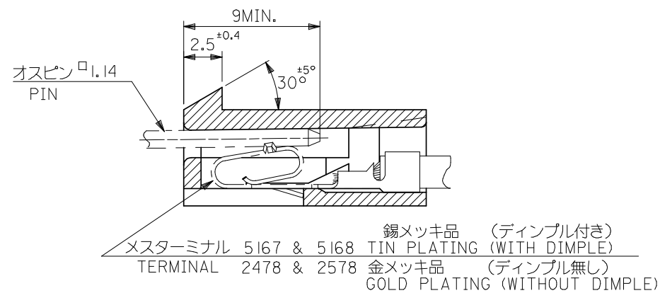
SECT. C-C
