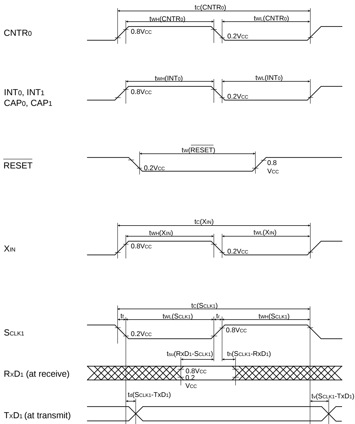
Fig. 107 Timing chart
