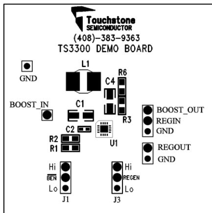
Figure 6. Top Layer #1
