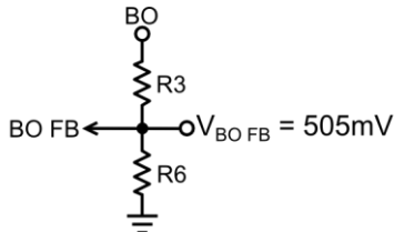
Figure 3: Setting the Boost Output Voltage with a Voltage Divider
