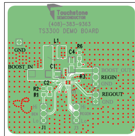
Figure 7. Top Layer #2
