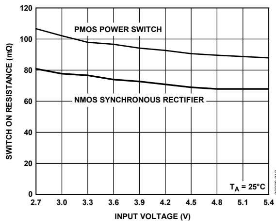
Figure 21. Switch On Resistance vs. Input Voltage—ADP2106 and ADP2107
