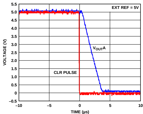
Figure 44. Hardware \overline{CLR}
