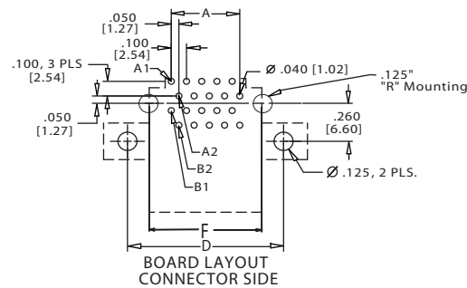
CARD LAYOUT
