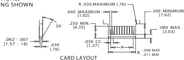
CARD LAYOUT
