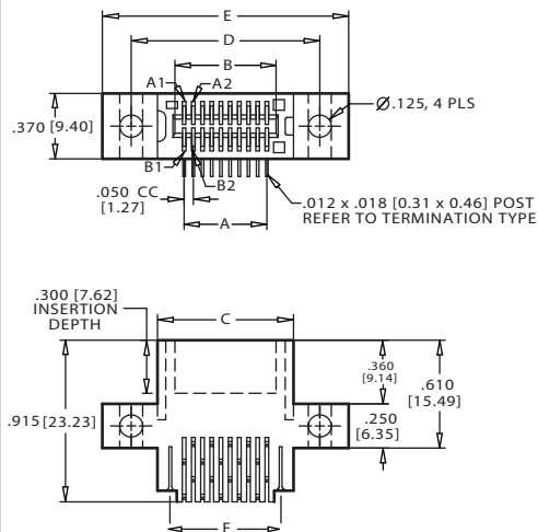
10 POSITIONS, (S) MOUNTING SHOWN
