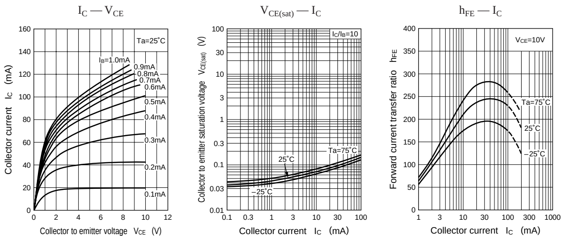
Characteristics charts of UN2214
