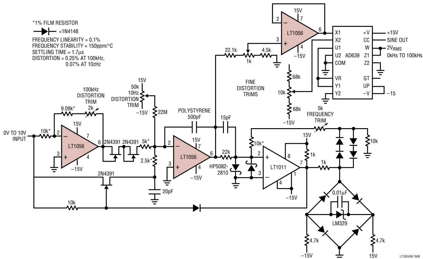
100kHz Voltage Controlled Oscillator
