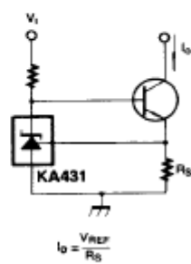
Figure 15. Constant-Current Sink
