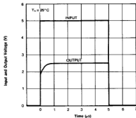
Figure 9. Pulse Response
