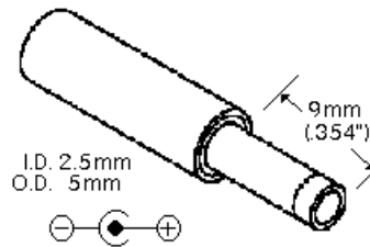
Figure 2. Power Input Power is applied to the 2.5mm connector. Power requirement 5 +/-10% VDC @250mA
