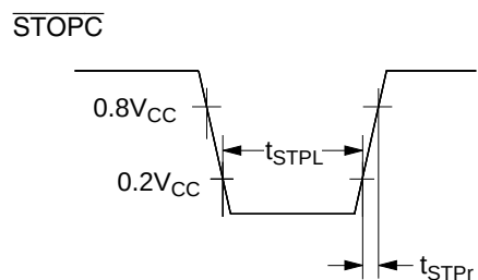
Figure 87 \overline{STOPC} Timing
