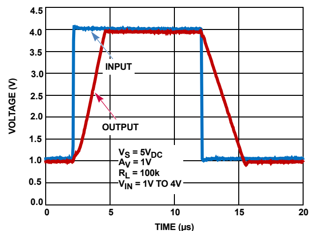
FIGURE 39. LARGE SIGNAL STEP RESPONSE (3V)
