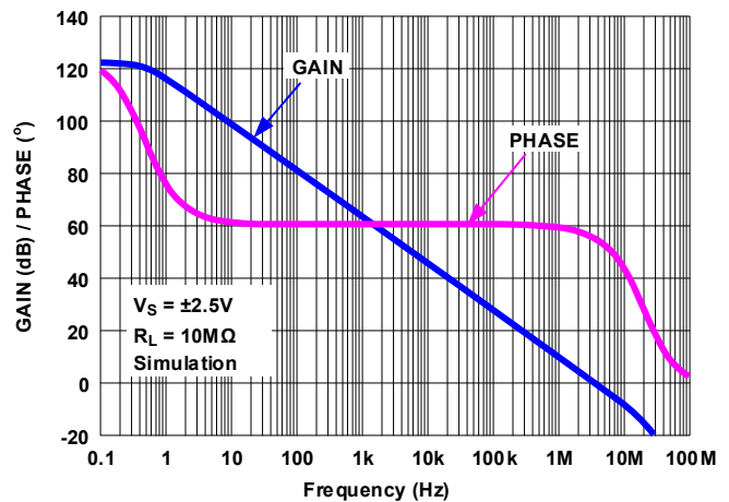
FIGURE 53. SIMULATED OPEN-LOOP GAIN, PHASE vs FREQUENCY
