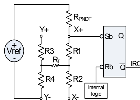
Figure 10. 4-wire pen detection circuitry
