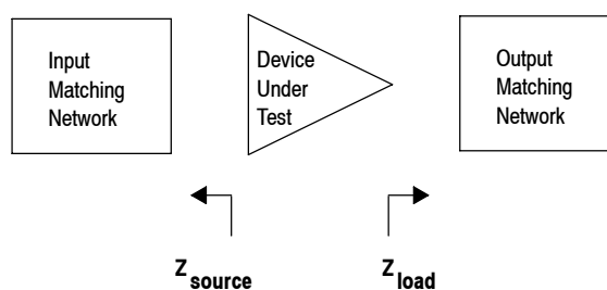
Figure 15. Series Equivalent Source and Load Impedance — 220 MHz
