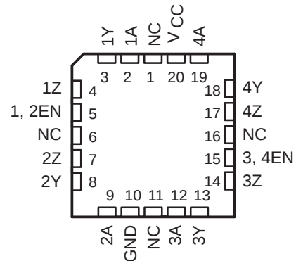
SN55ALS194 . . . FK PACKAGE (TOP VIEW)
