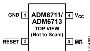
Figure 4. Pin Configuration
