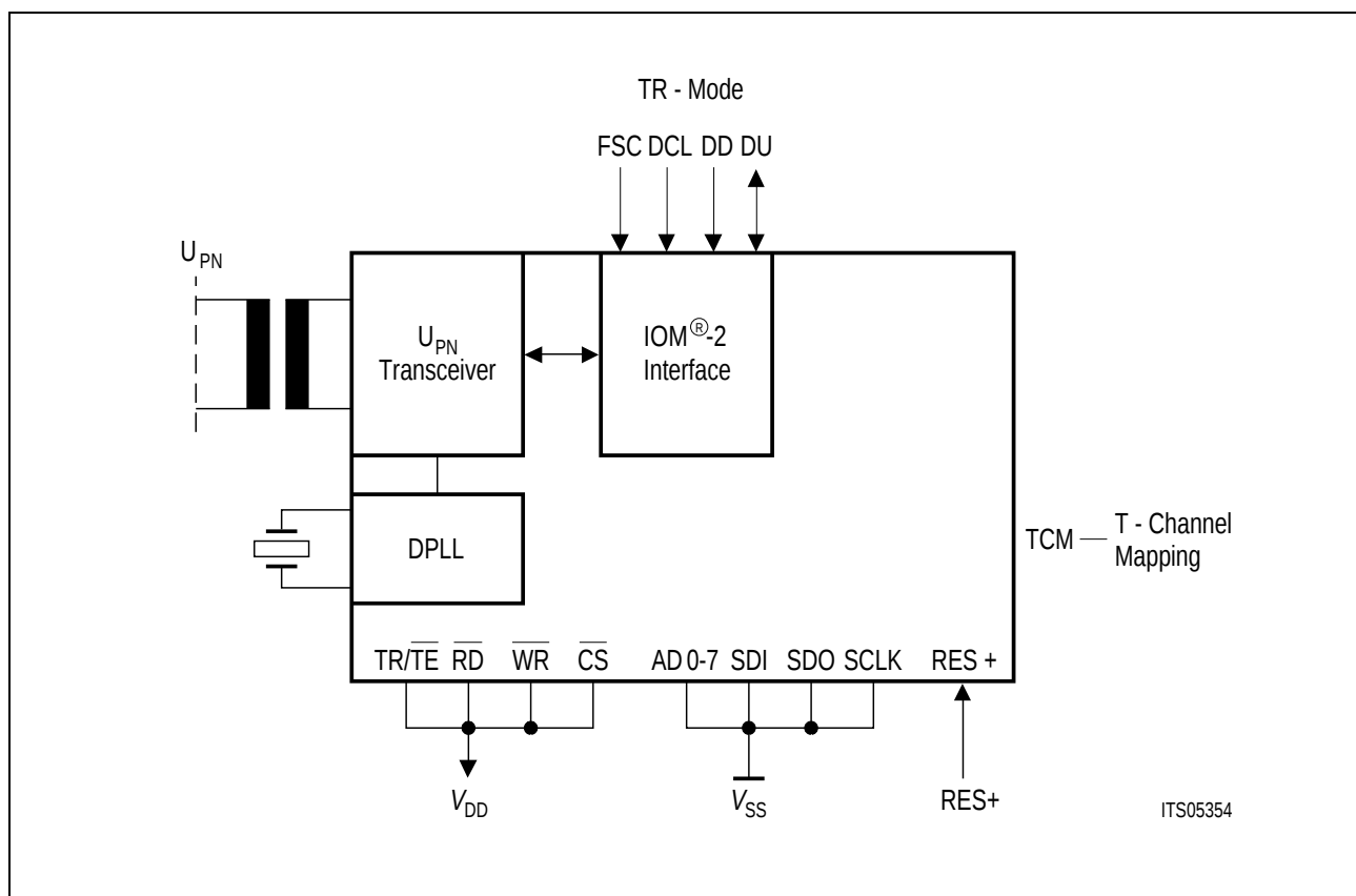
Figure 35 Device Architecture in TR-Mode
