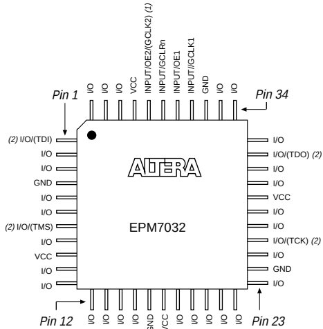
44-Pin PQFP
