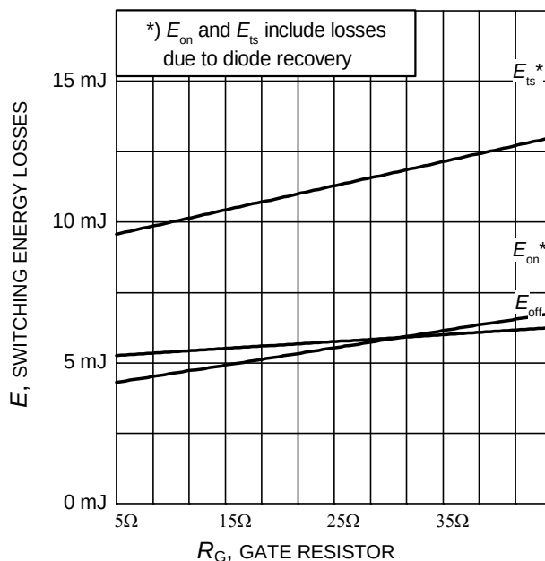
Figure 14. Typical switching energy losses as a function of gate resistor (inductive load, T_J=150^\circ\text{C} , V_{CE}=600\text{V} , V_{GE}=0/15\text{V} , I_C=40\text{A} , Dynamic test circuit in Figure E)
