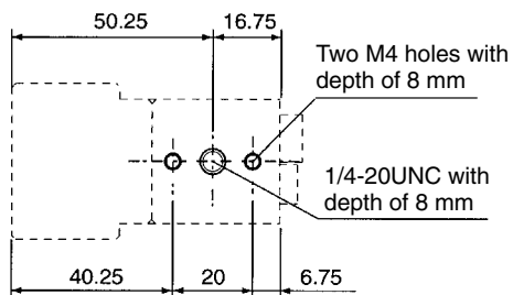
Mounting dimensions
