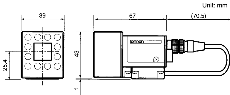
Mounting dimensions
