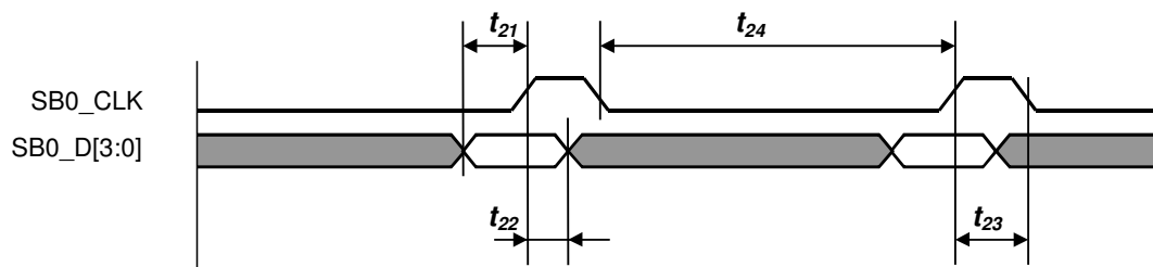
Figure 3.10: Tx Sideband Data Interface; Low Speed Upstream
