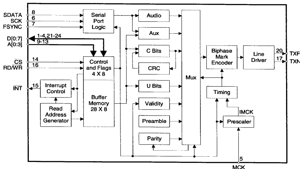
Figure 4. CS8403A Block Diagram
