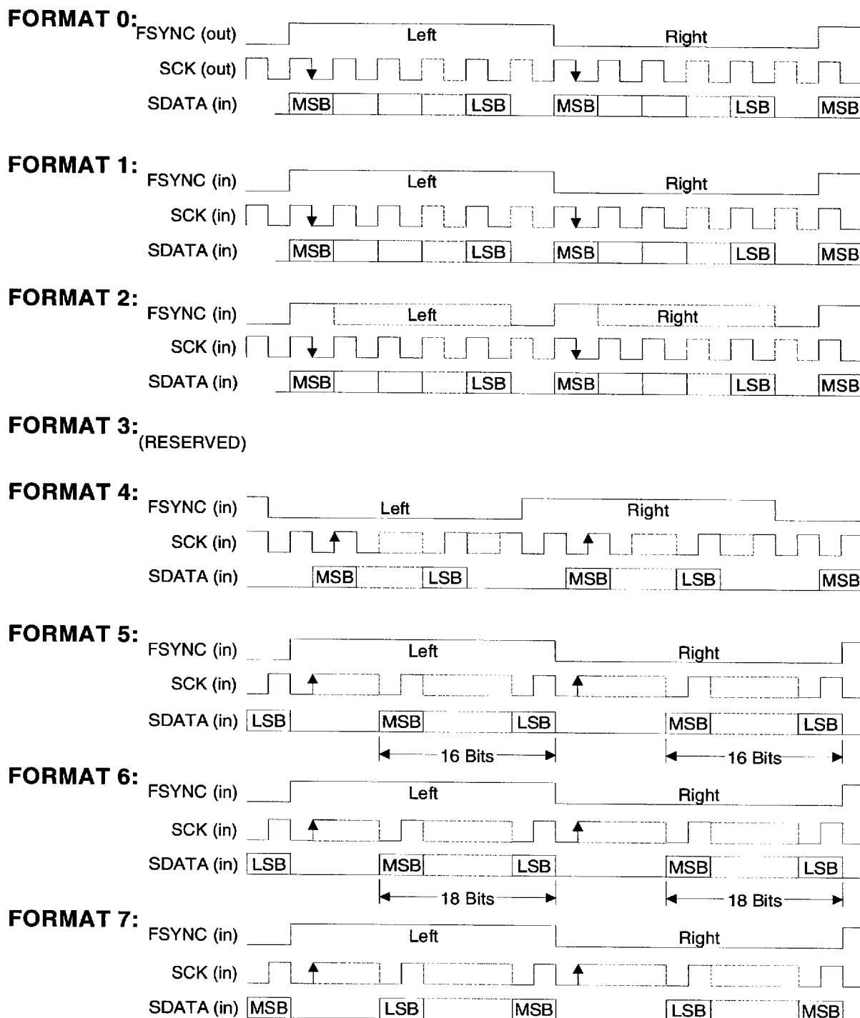
Figure 16. CS8404A Audio Serial Port Formats
