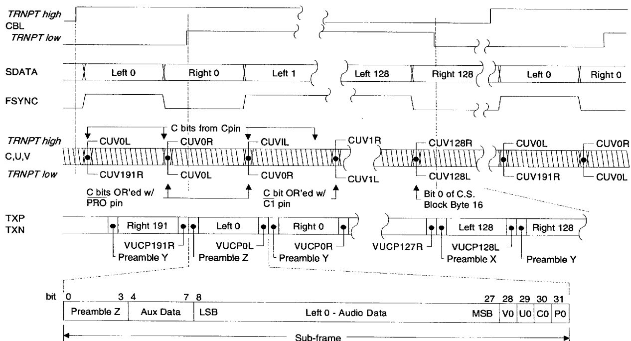
Figure 17. CBL and Transmitter Timing
