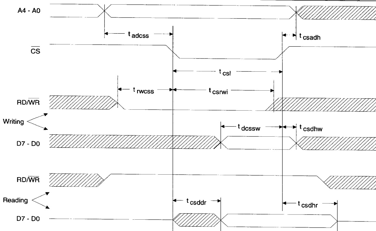
CS8403A Parallel Port Timing
