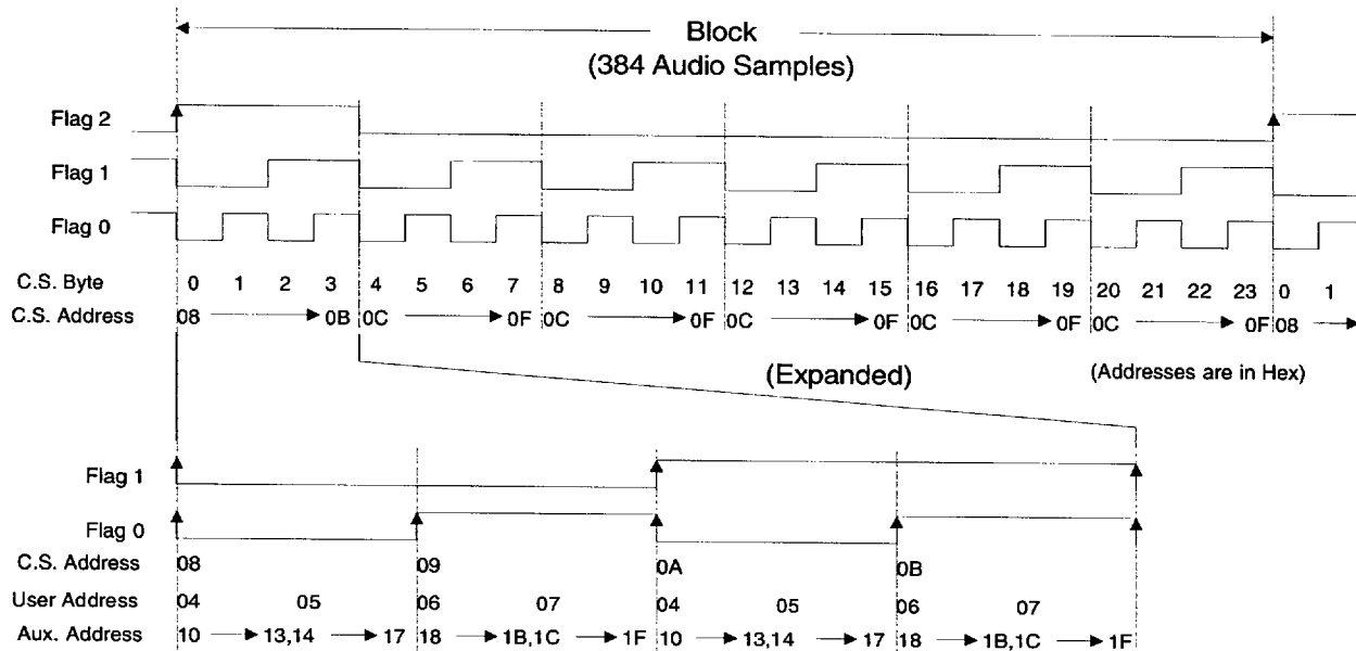
Figure 13. CS8403A Buffer Memory Read Sequence - MODE 1
