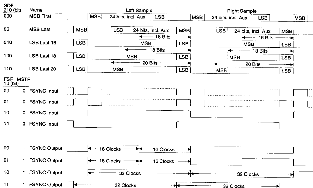
Figure 10. CS8403A Serial Port SDATA and FSYNC Timing
