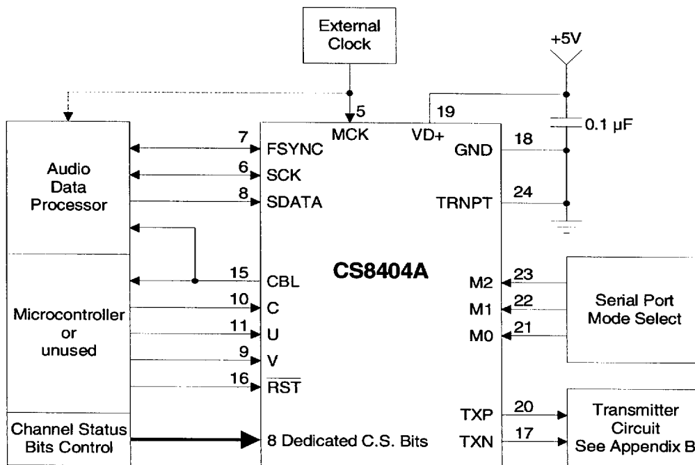
Figure 2. CS8404A Professional & Consumer Modes Typical Connection Diagram
