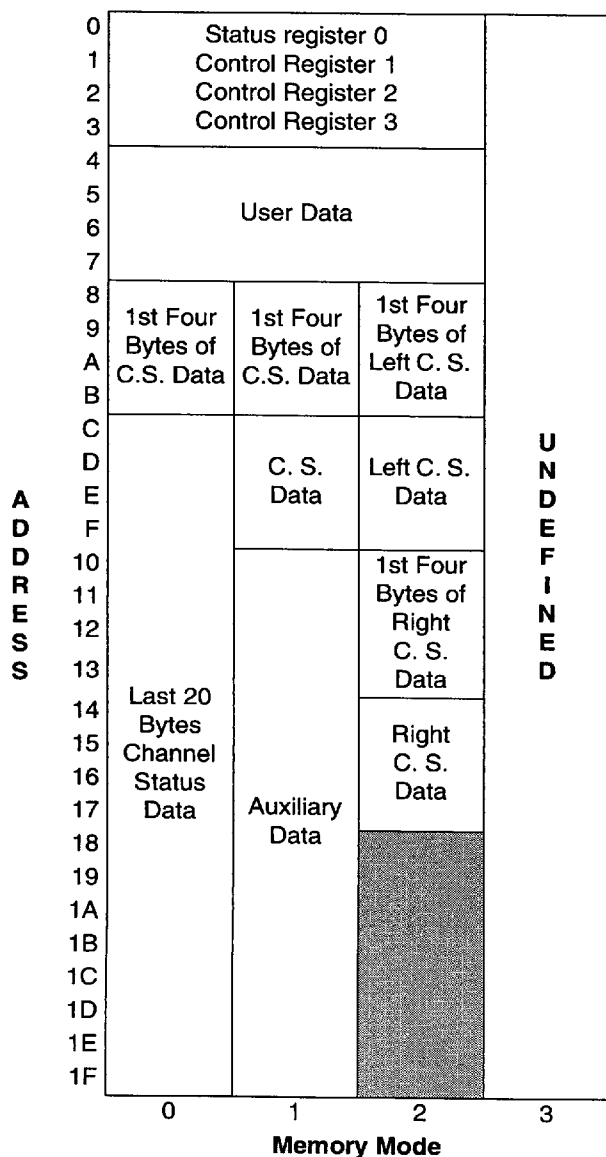
Figure 5. CS8403A Buffer Memory Modes
