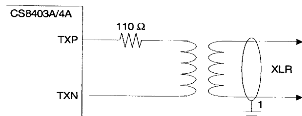
Figure A1. Professional Output Circuit
