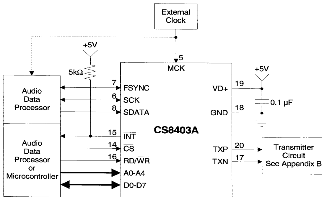
Figure 1. CS8403A Typical Connection Diagram
