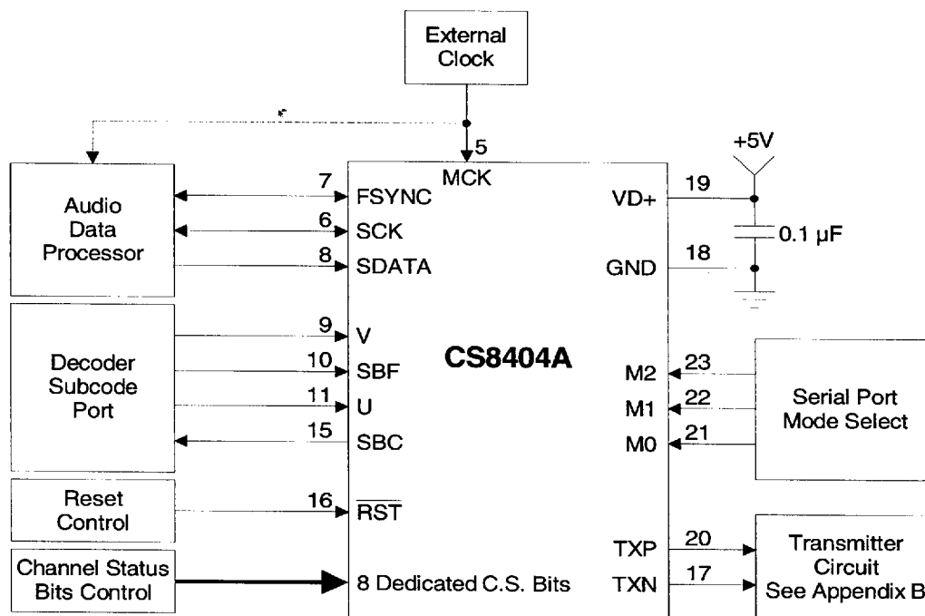
Figure 3. Consumer CD Submode Typical Connection Diagram
