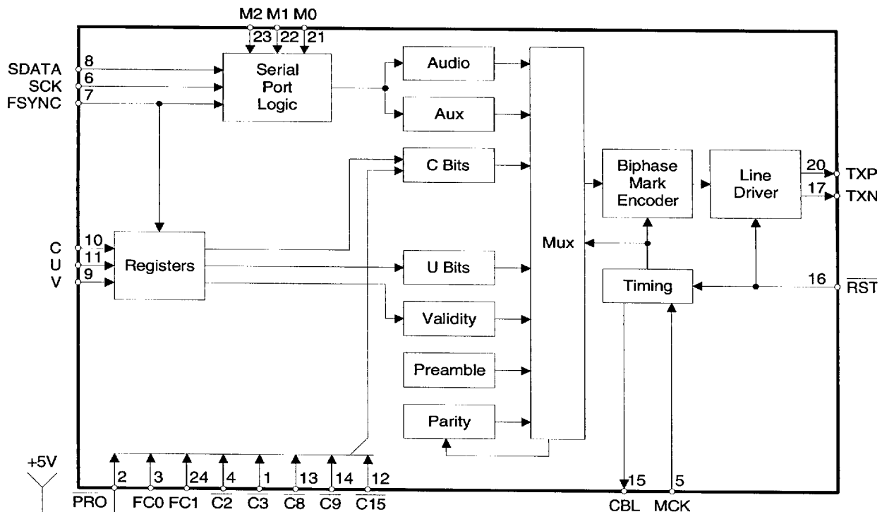
Figure 20. CS8404A Block Diagram - Consumer Mode
