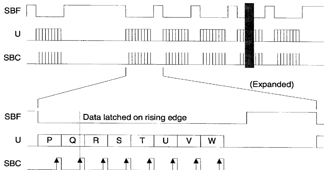
Figure 22. CD Subcode Port Timing
