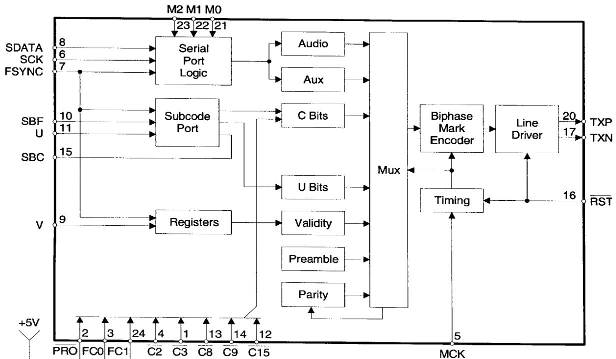
Figure 21. CS8404A Block Diagram - Consumer Mode, CD Submode
