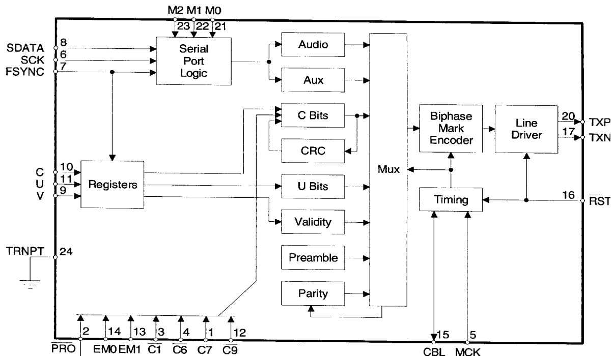
Figure 19. CS8404A Block Diagram - Professional Mode
