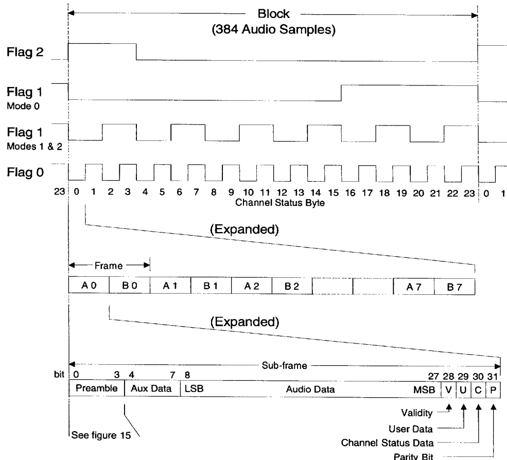
Figure 11. CS8403A Status Register Flag Timing
