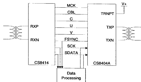
Figure 18. Transparent Mode Interface
