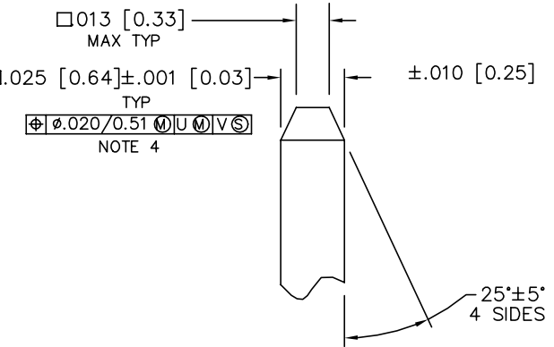
DETAIL P SCALE 5:1 TYP BOTH ENDS
