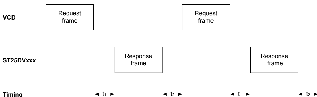
Figure 32. ST25DVxxx protocol timing
