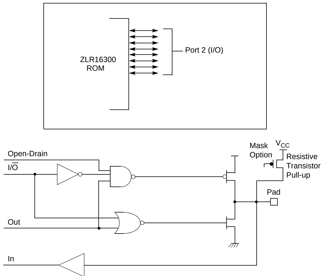
Figure 6. Port 2 Configuration
