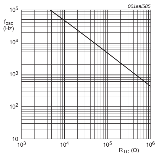
b. R_{TC} curve at C_{TC} = 1 \text{ nF} ; R_S = 2 \text{ R}_{TC} .
