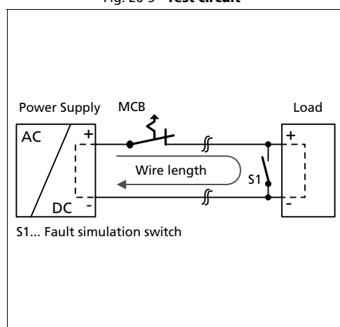
Fig. 26-5 Test circuit
