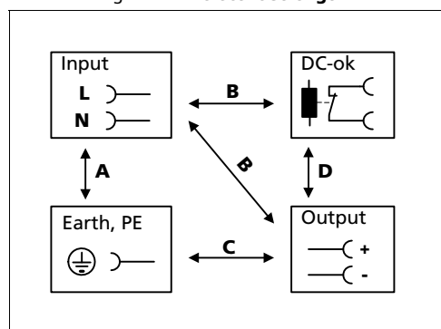
Fig. 21-1 Dielectric strength
