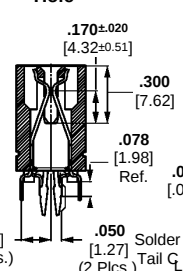
Section L-L
