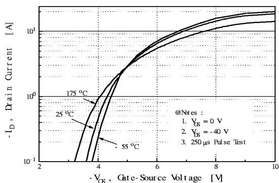
Fig 2. Transfer Characteristics
