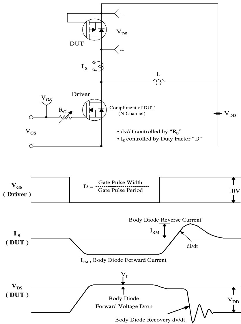
Fig 15. Peak Diode Recovery dv/dt Test Circuit & Waveforms
