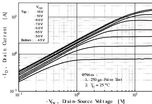
Fig 1. Output Characteristics
