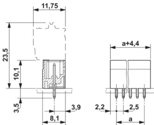
Dimensioned drawing
