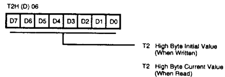
Figure 34. Counter Timer 2 Register High Byte (06H: Read/Write)
