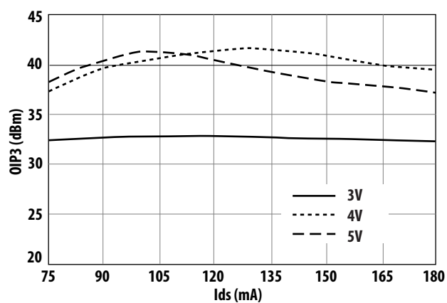
Figure 7. OIP3 vs. I_{ds} and V_{ds} at 900 MHz
