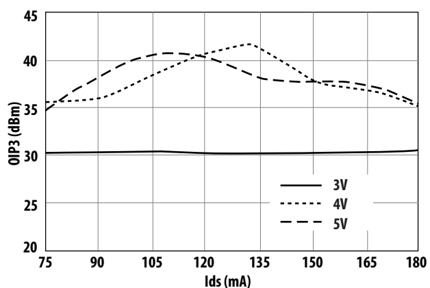
Figure 9. OIP3 vs. I_{ds} and V_{ds} at 3.9 GHz
