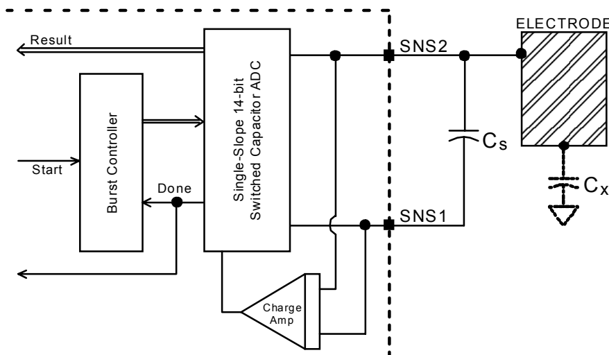
Figure 1-3 Internal Switching & Timing
