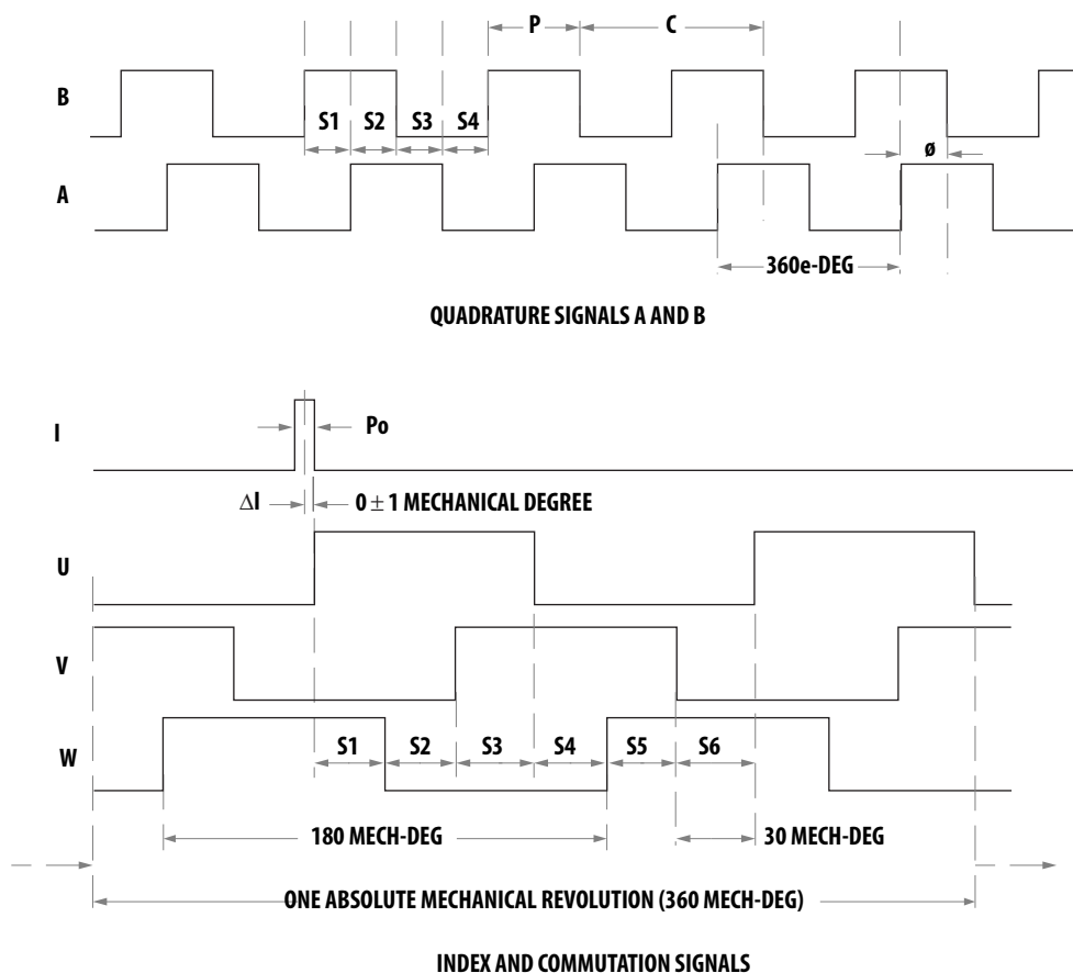
Figure 6. Output waveform specification of 2 pole-pairs (4 poles) for counter clockwise rotation, viewed from the top
